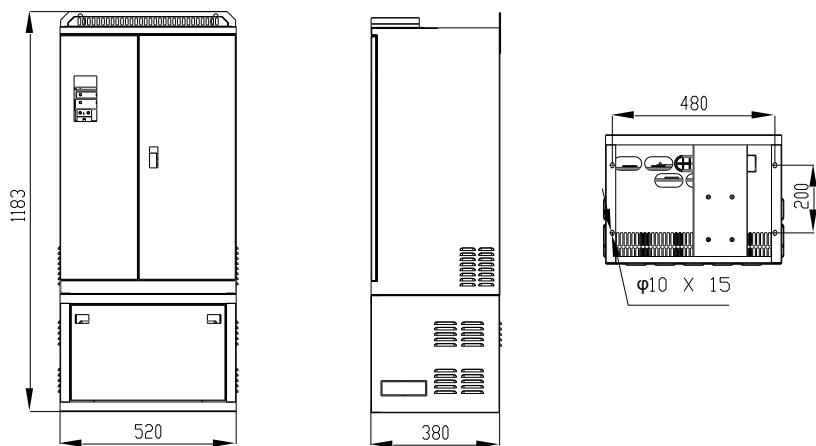
图 2-4 1850G/2000P~2500G/2800P (T4/T5 电压等级)落地安装示意图
